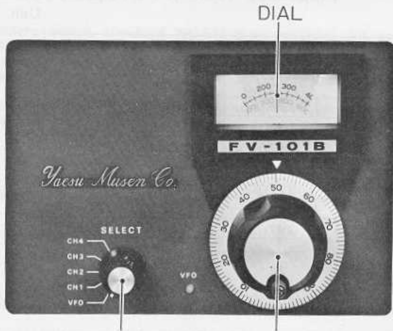
SELECT SWITCH TUNING KNOB
